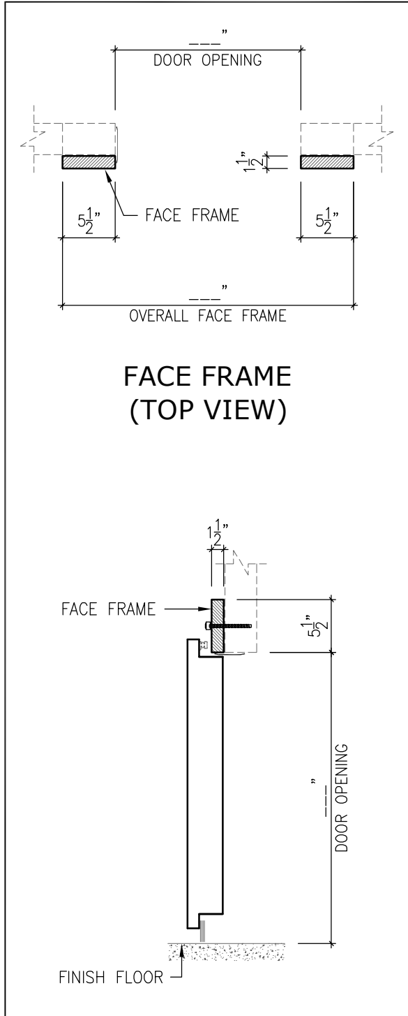
FACE FRAME (SIDE VIEW)
